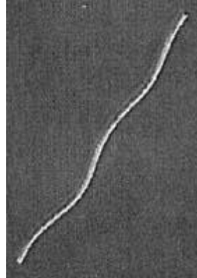
Methanobacterium thermoautotrophicum
