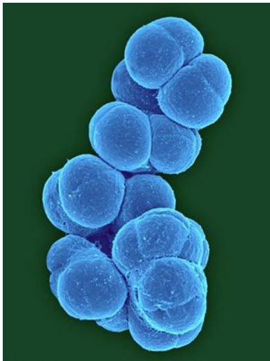
Methanosarcina barkeri
