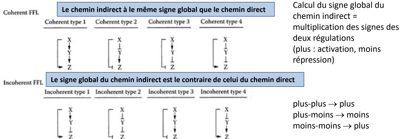
FIGURE 4.3 The eight sign combinations (types) of feed-forward loops. Arrows denote activation and \perp symbols denote repression.
